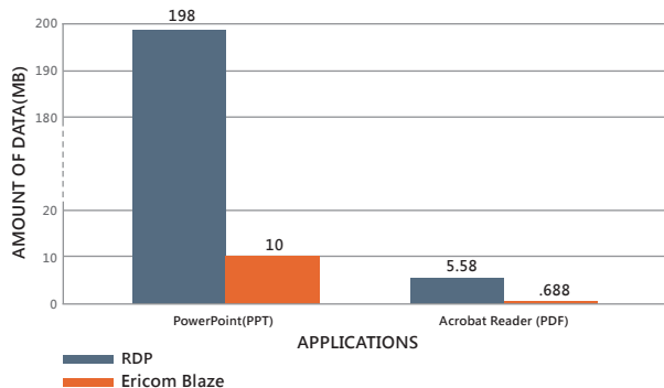
Chart 1: RDP versus Ericom Blaze: The total amount of data that was transferred following compression
